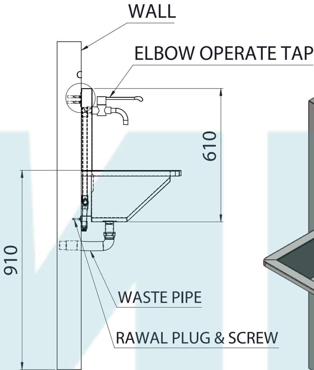
SIDE VIEW
