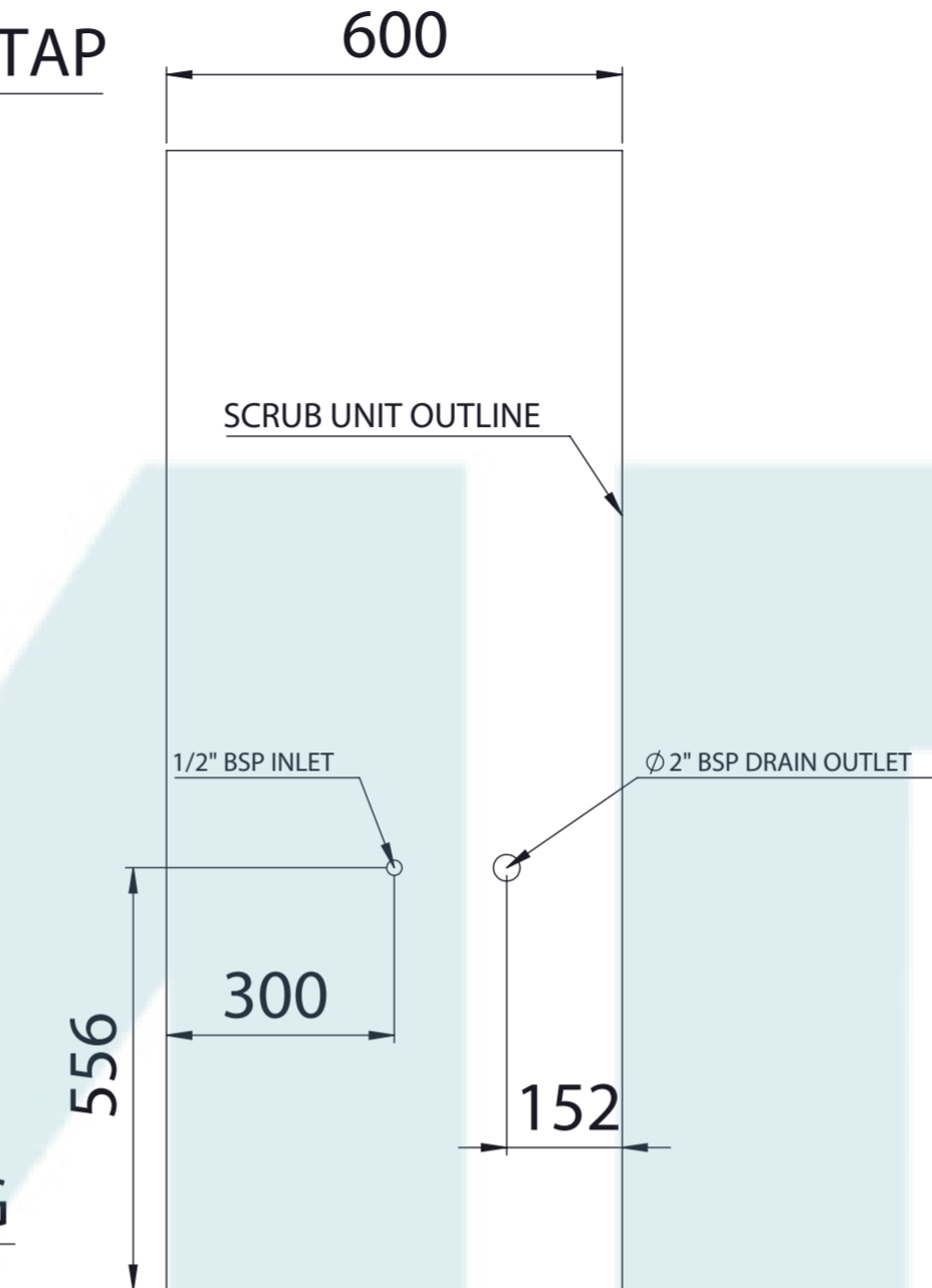
WALL PLUMBING DIAGRAM
