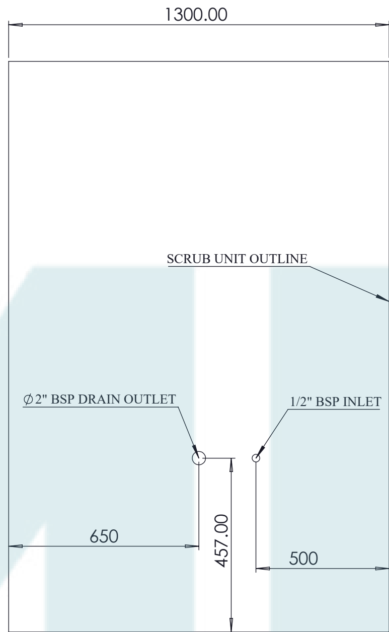
WALL PLUMBING DIAGRAM
