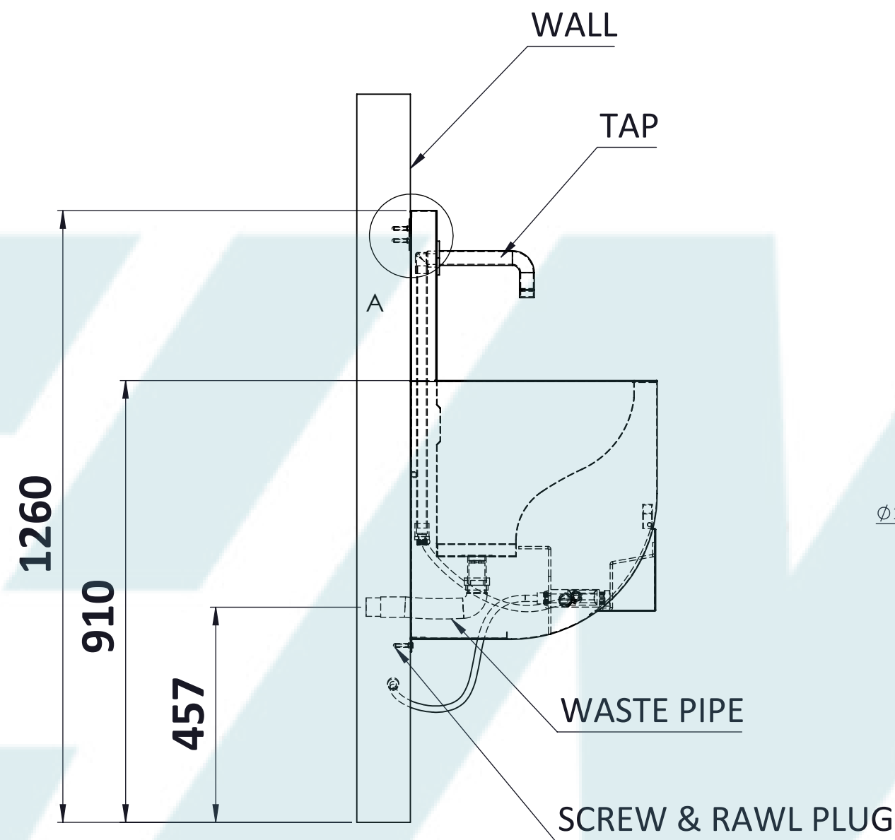
SIDE VIEW
