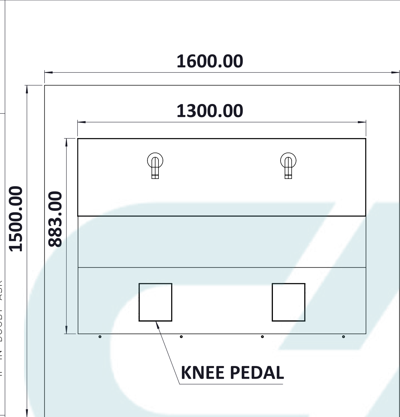
FRONT VIEW
