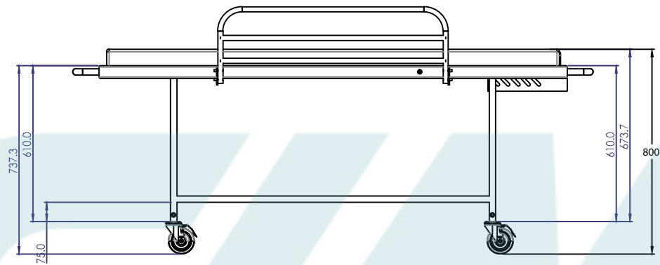
FRONT VIEW
