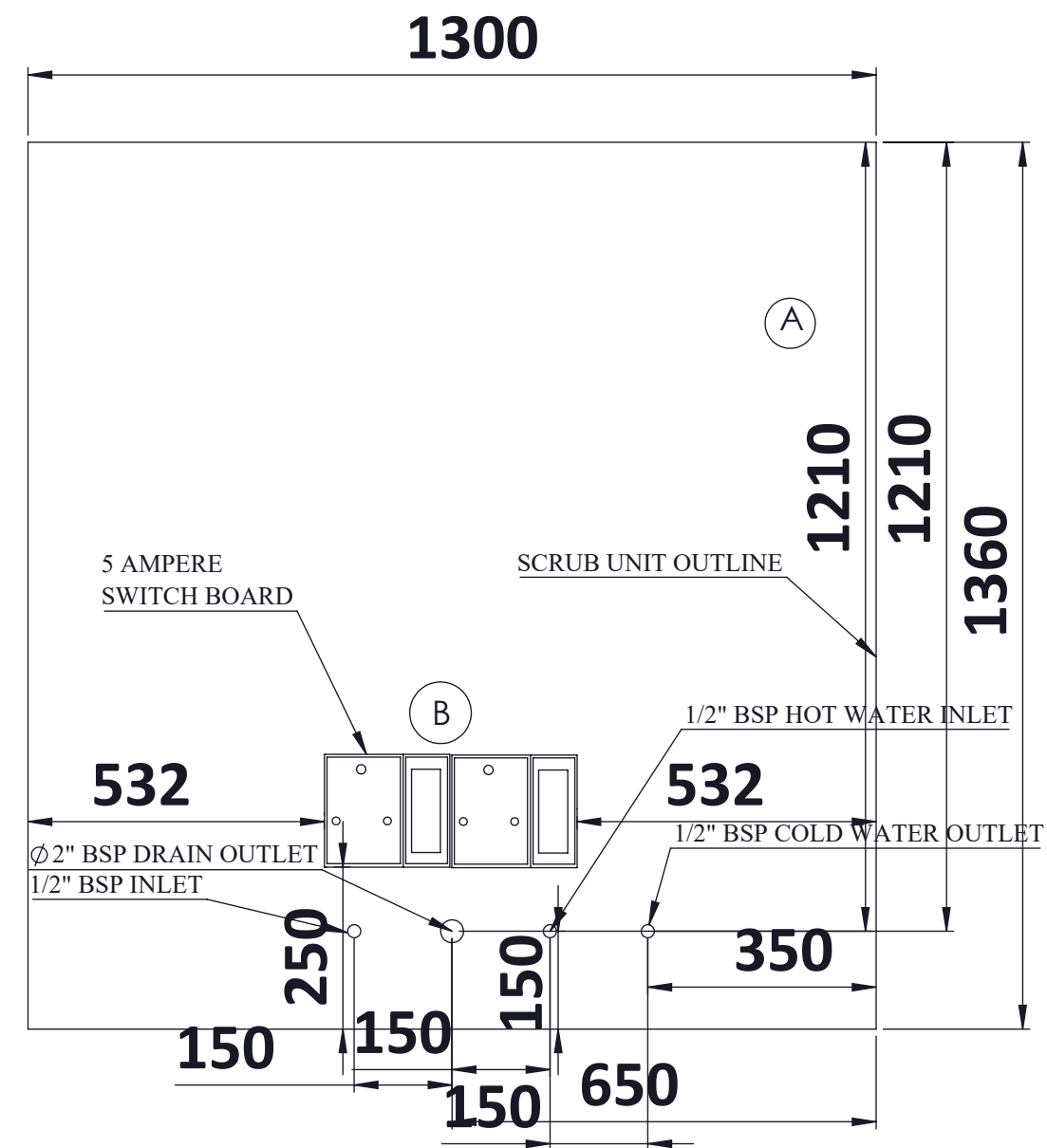
WALL PLUMBING DIAGRAM
