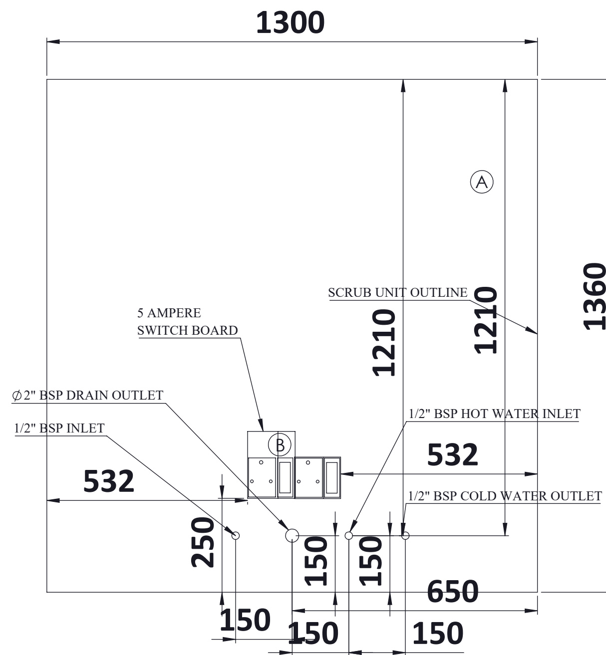
WALL PLUMBING DIAGRAM
