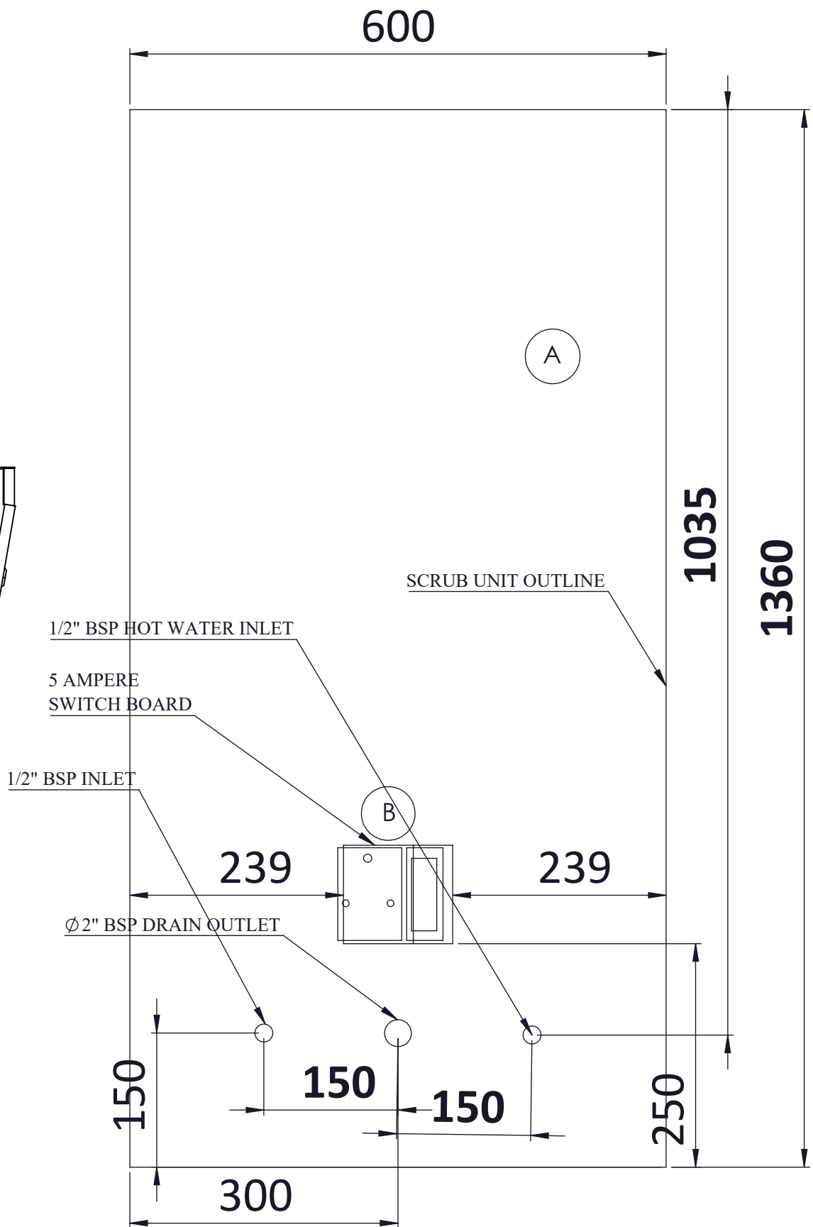
WALL PLUMBING DIAGRAM
