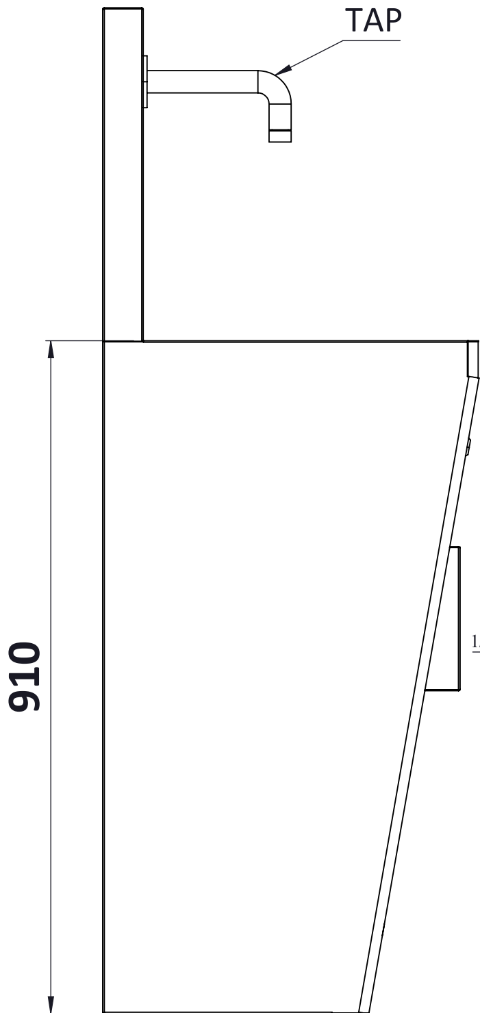
SIDE VIEW
