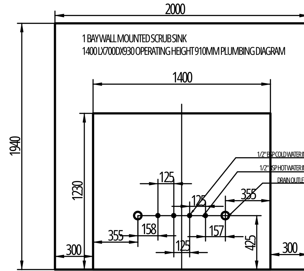
WALL PLUMBING DIAGRAM
