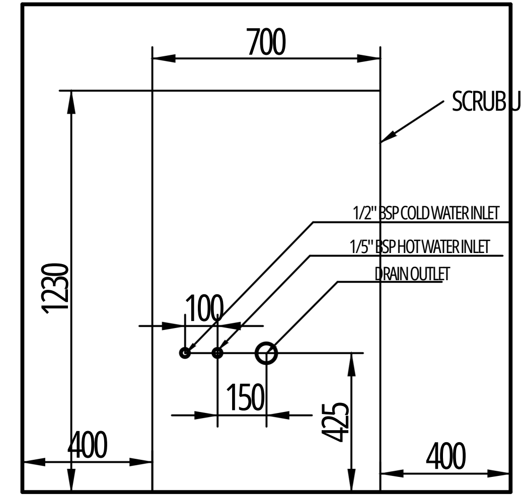
WALL PLUMBING DIAGRAM
