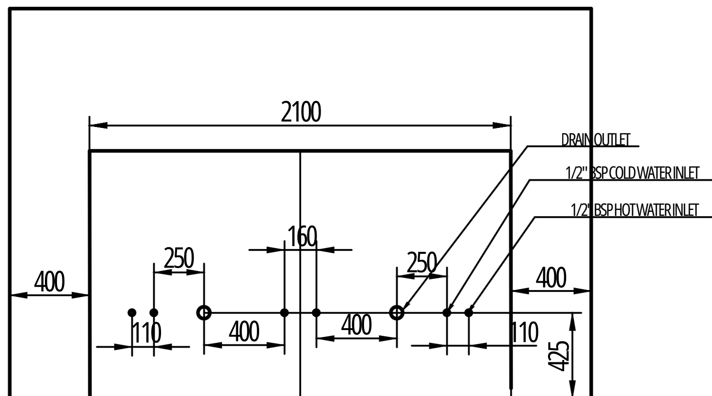
WALL PLUMBING DIAGRAM
