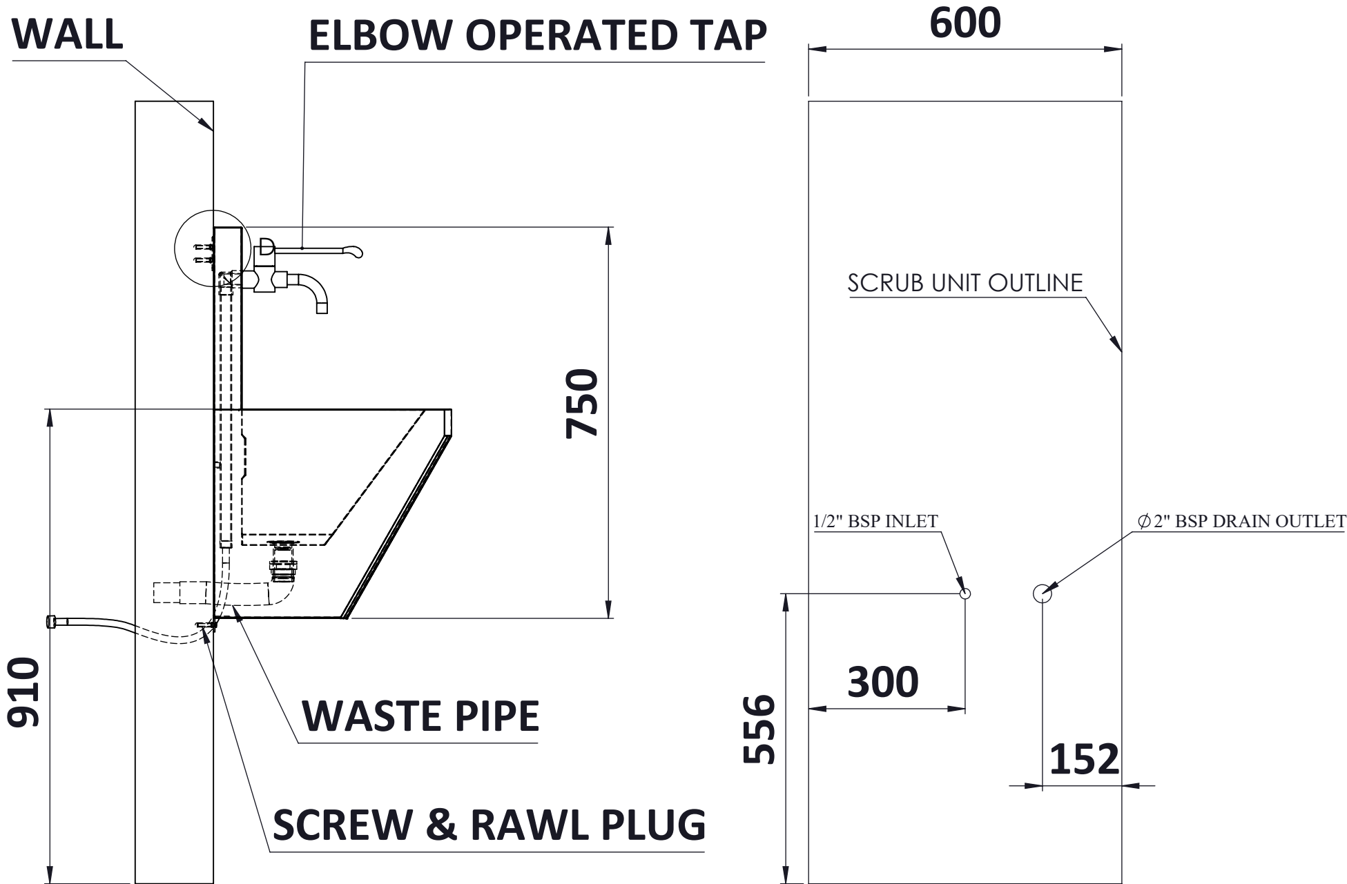
SIDE VIEW
