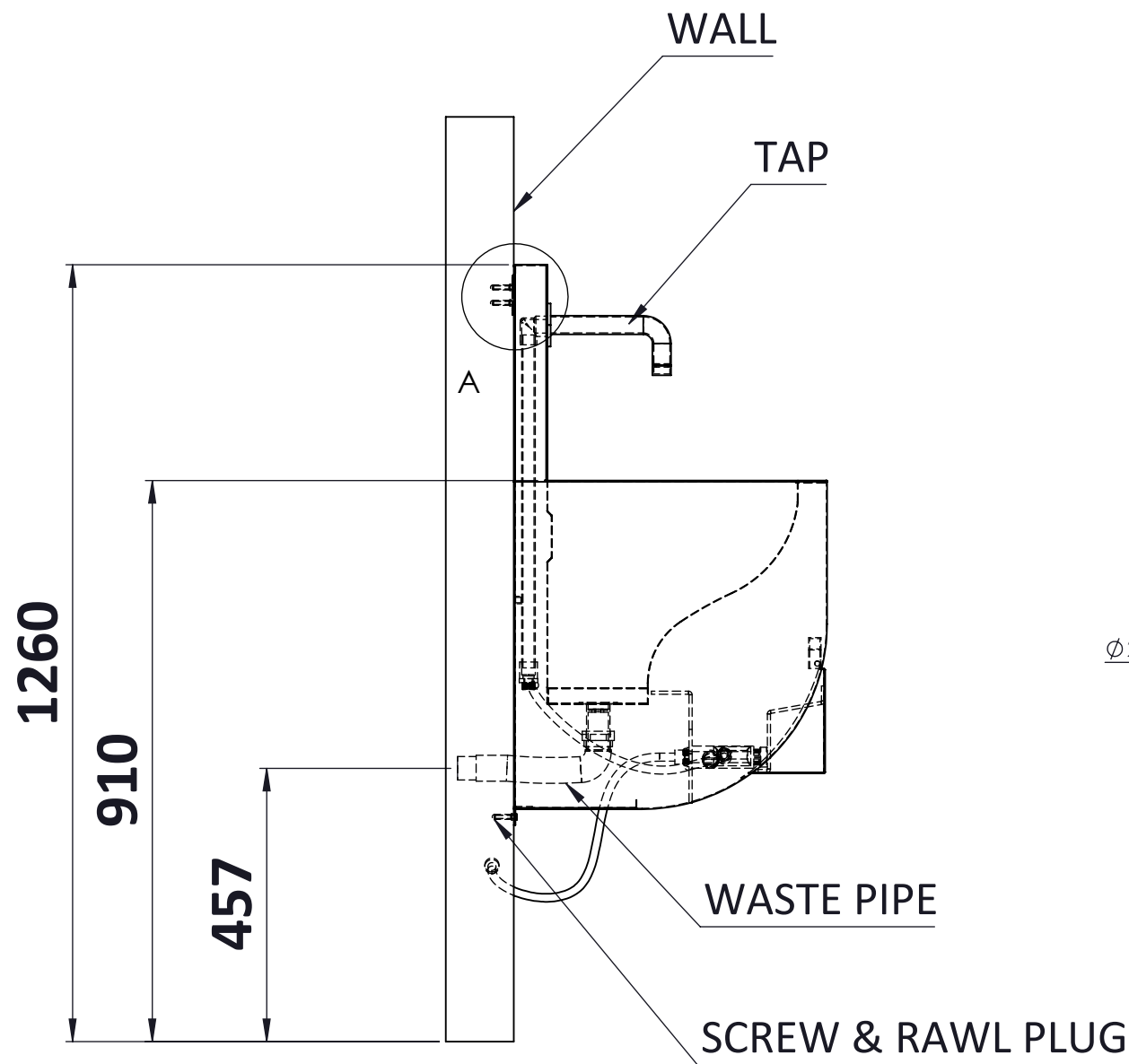
SIDE VIEW
