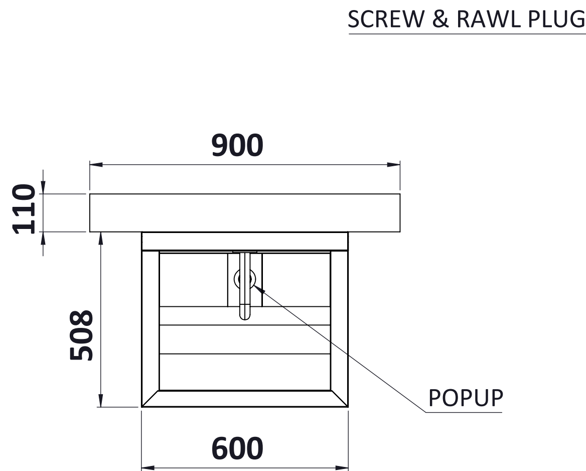
TOP VIEW
