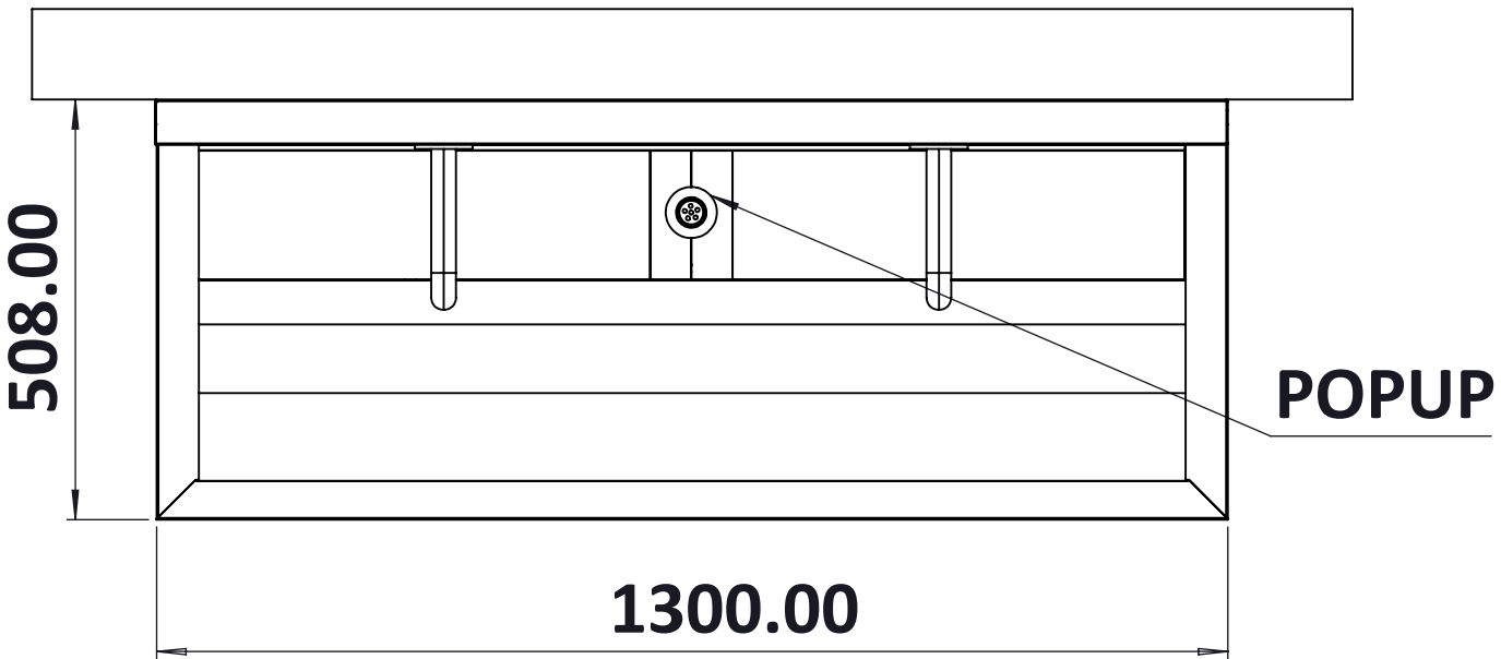
TOP VIEW
