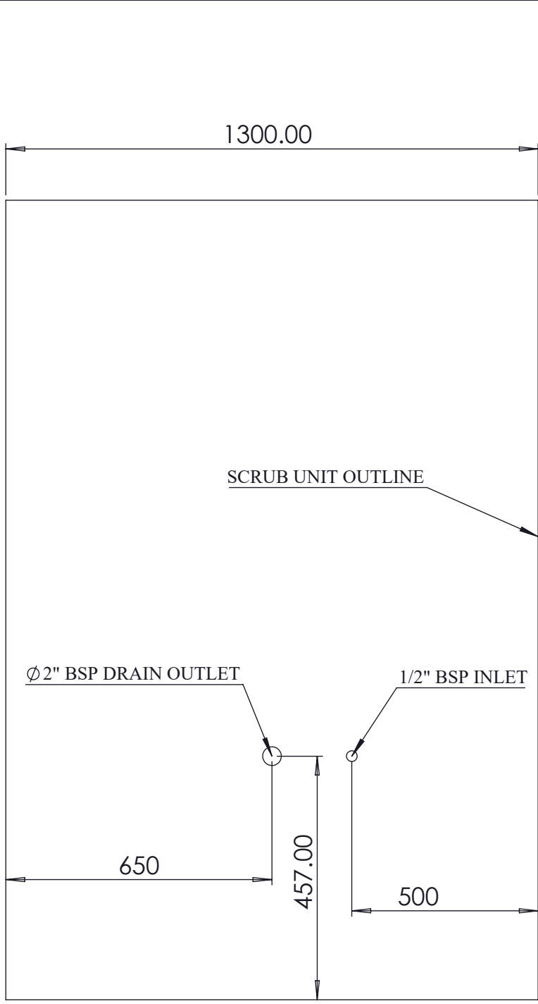
WALL PLUMBING DIAGRAM
