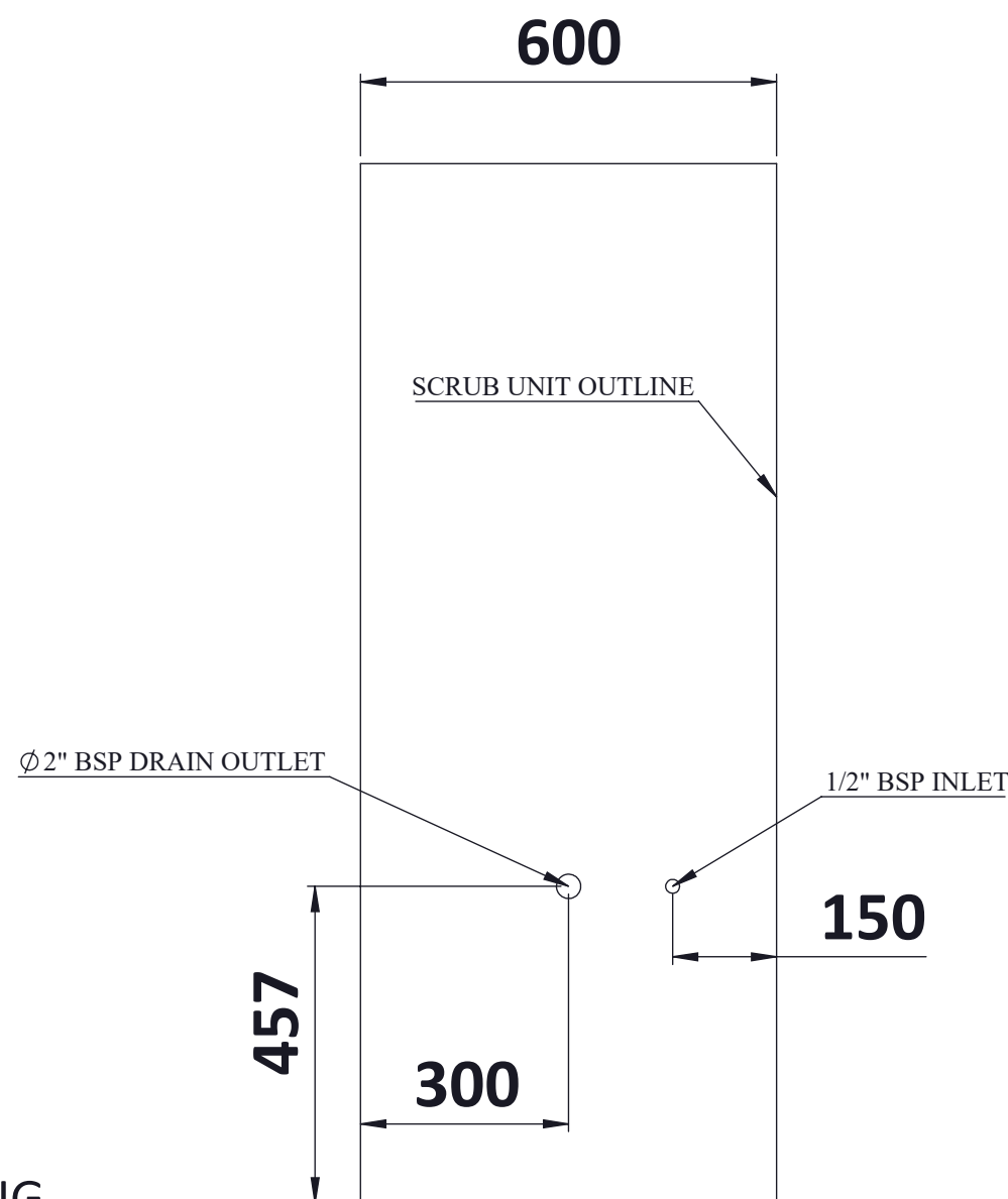
WALL PLUMBING DIAGRAM
