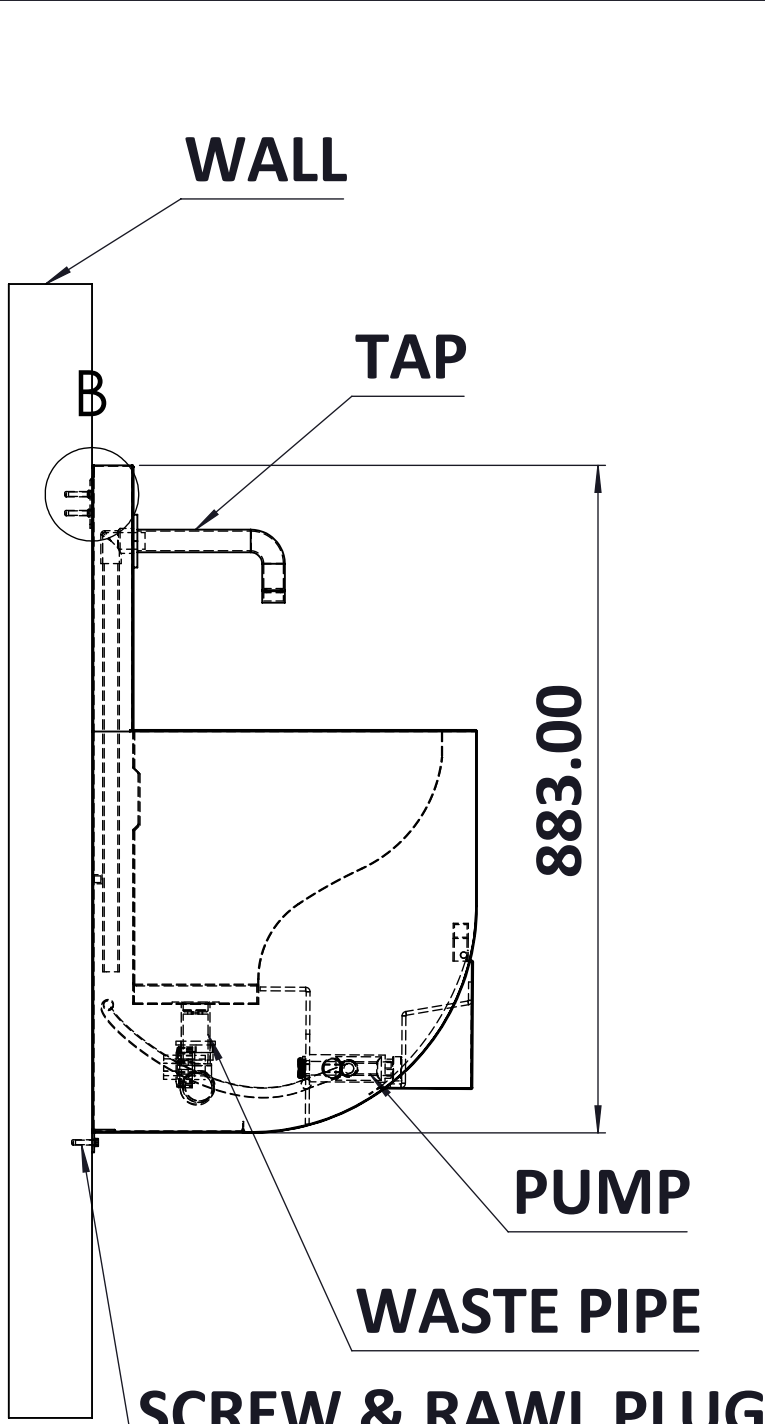
SIDE VIEW
