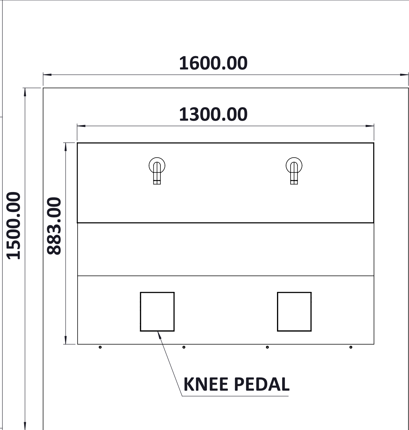
FRONT VIEW
