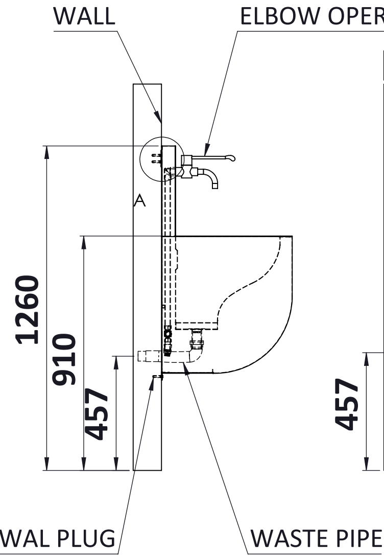
SIDE VIEW
