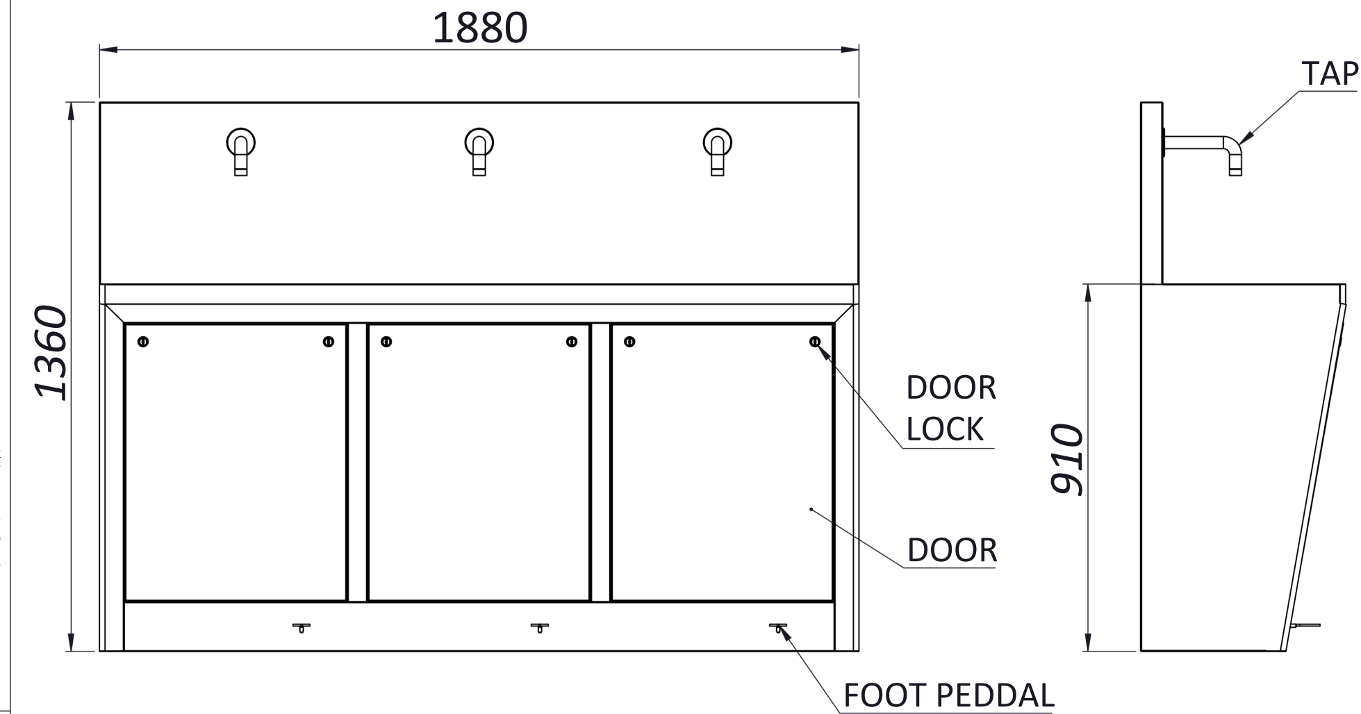
SIDE VIEW
