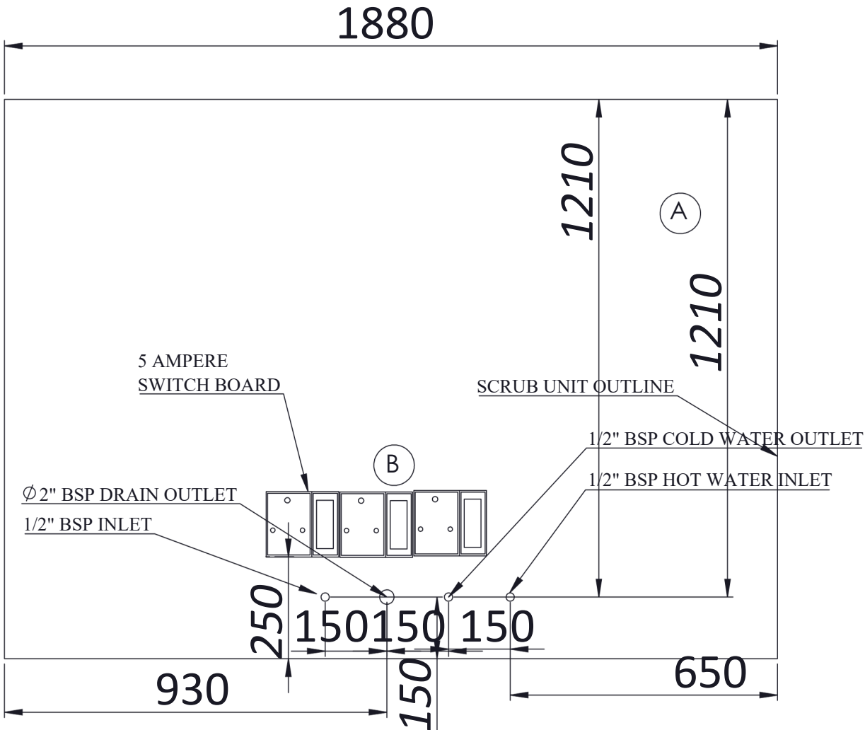
WALL PLUMBING DIAGRAM
