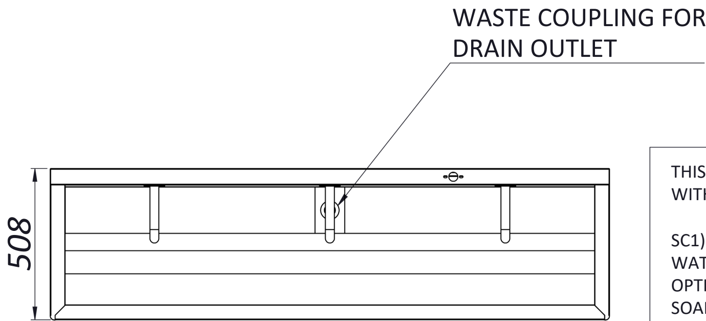
TOP VIEW
