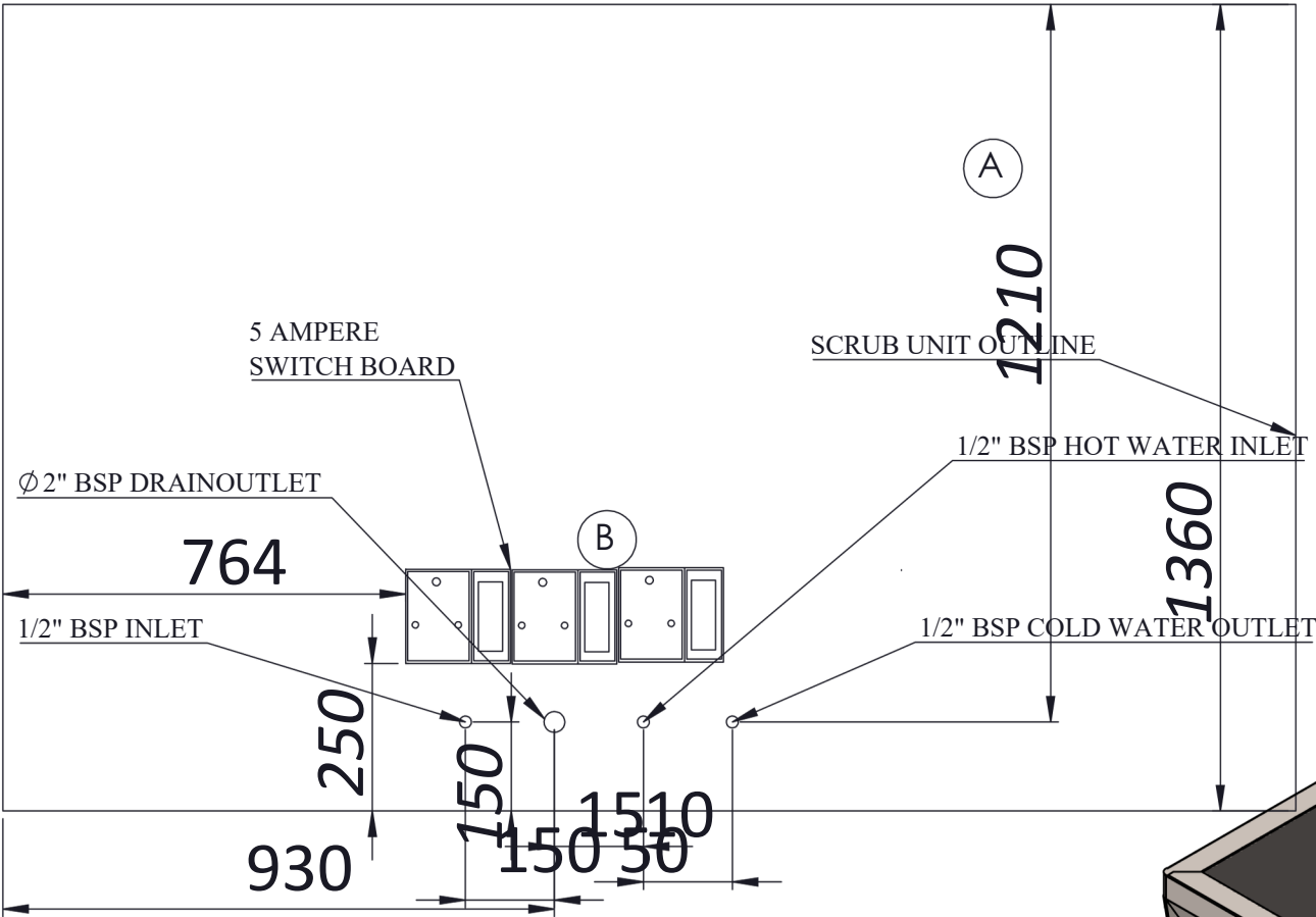
WALL PLUMBING DIAGRAM
