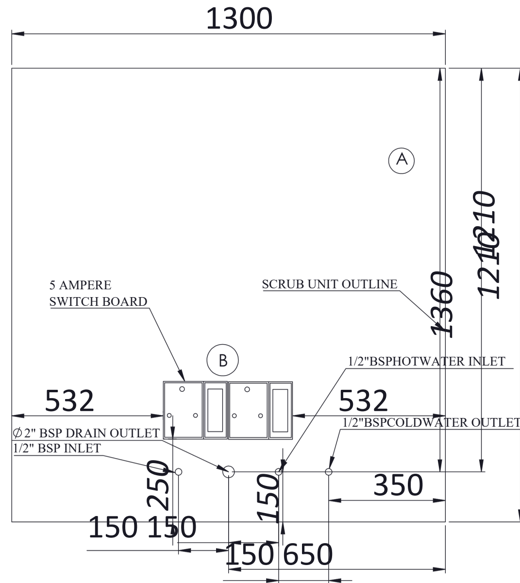
WALL PLUMBING DIAGRAM
