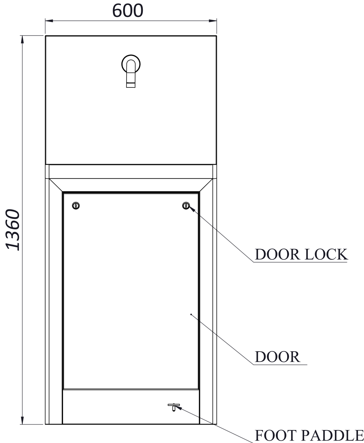
FRONT VIEW
