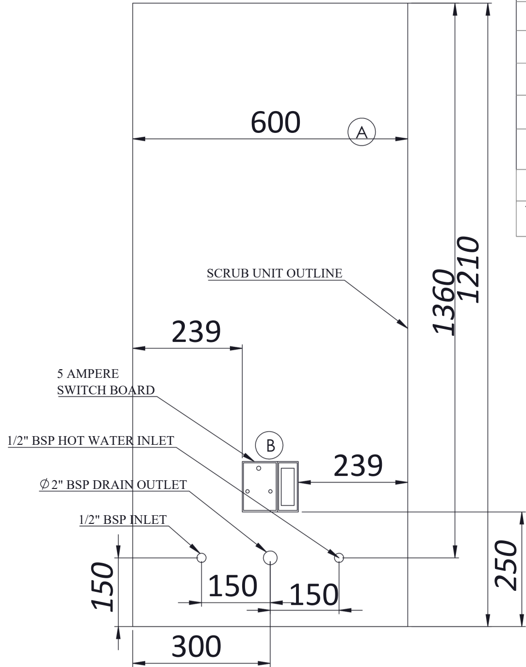
WALL PLUMBING DIAGRAM
