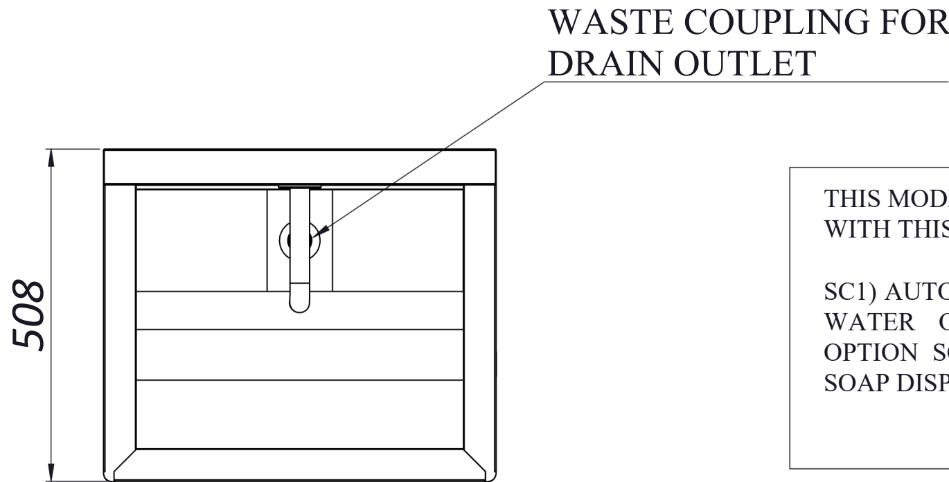
TOP VIEW
