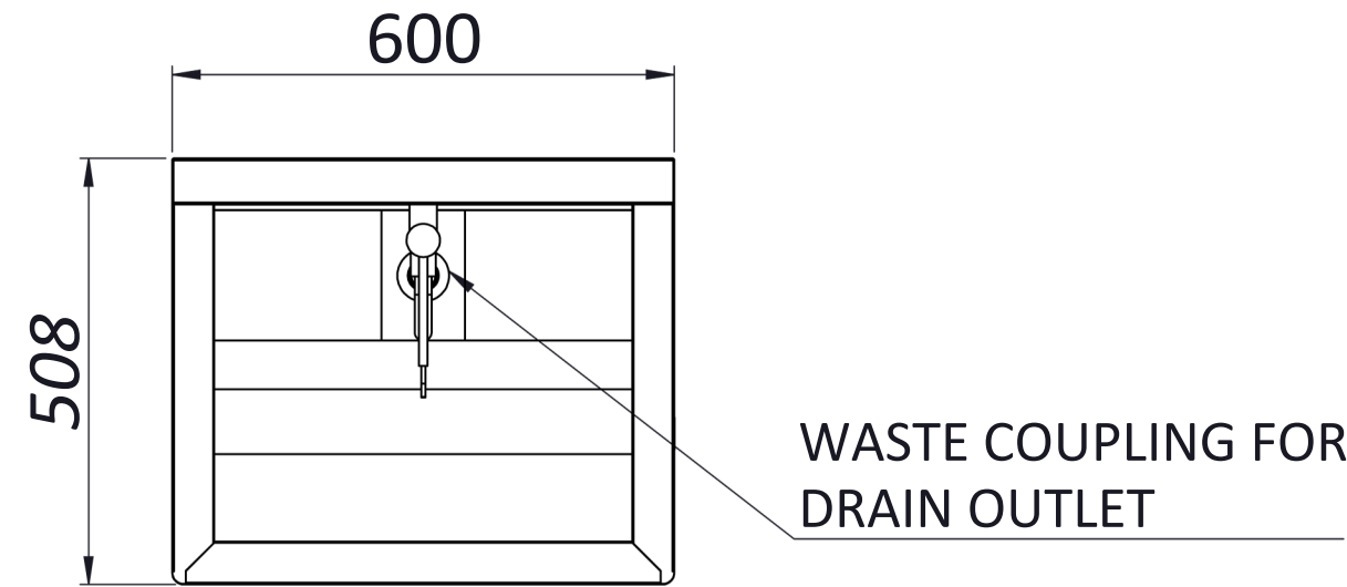
TOP VIEW
